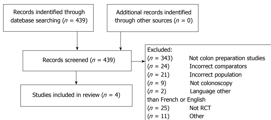
Figure 1 STROBE diagram.
